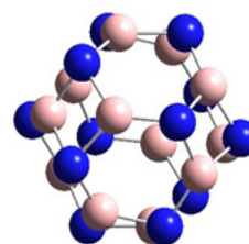
B_{12}N_{12}
