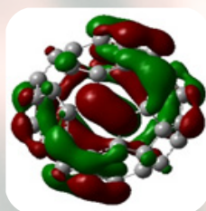
HOMO-c 60
