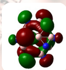
HOMO-B 12 N 12
