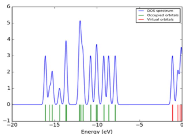
B 12 N 12
